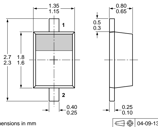
Fig 15. Package outline SOD323F (SC-90)
